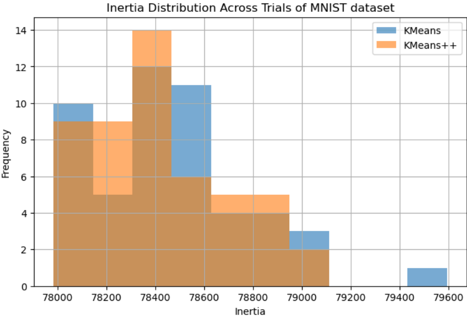
Figure 7: Bar graph of inertia distribution across 50 runs on MNIST
