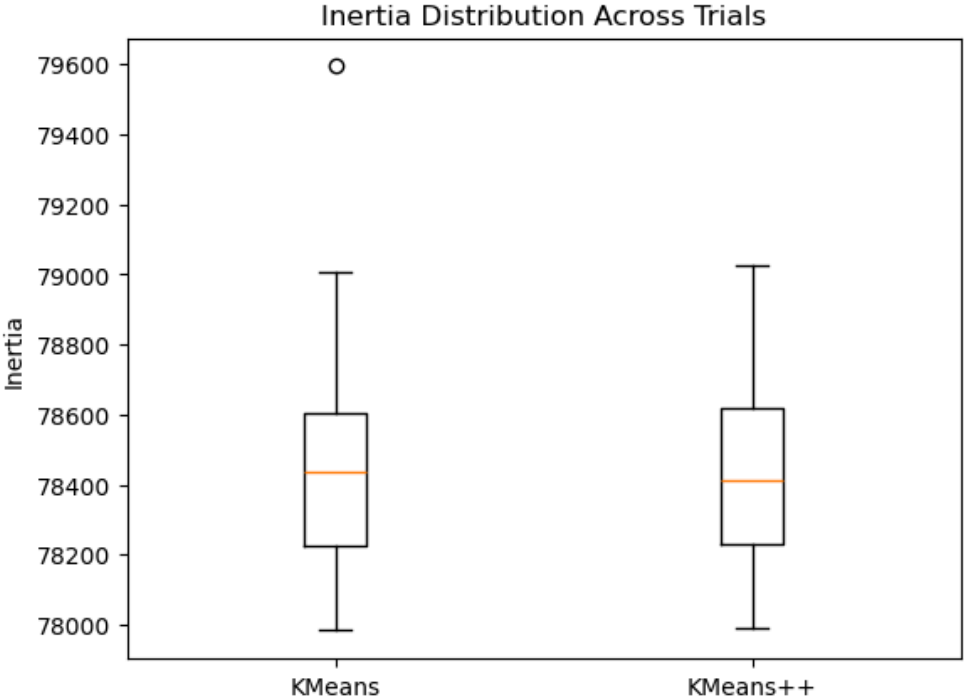
Figure 6: Box plot of inertia distribution across 50 runs on MNIST
